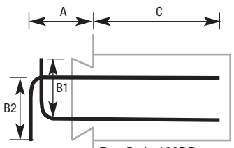
TYPE LJ: Double Angle Hook Bar
