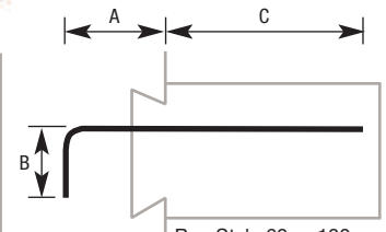
TYPE L: L Shaped Hook Bar
