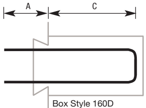
TYPE AU: Reverse U Shaped Bar
