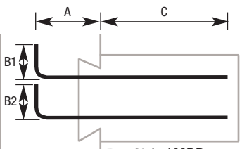
TYPE LL: Double L Shaped Hook Bar
