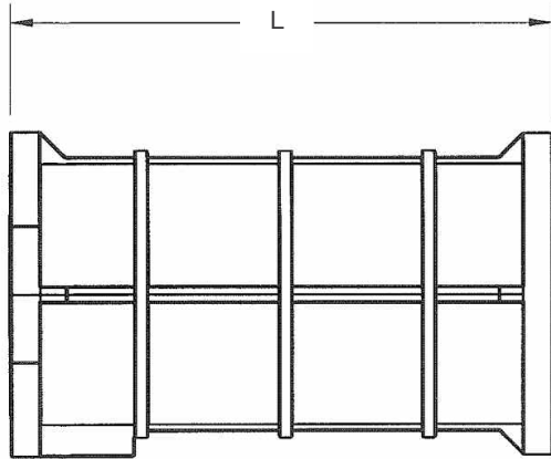
Threaded Socket Dimensions
