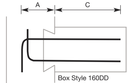
TYPE LJ: Double Angle Hook Bar
