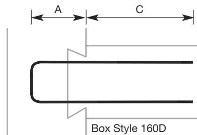
TYPE U: U Shaped Bar
