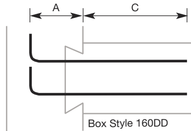
TYPE LL: Double L Shaped Hook Bar
