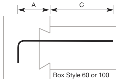
TYPE L: L Shaped Hook Bar
